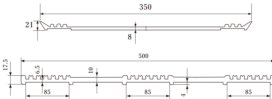
Rubber Profile Diagram
